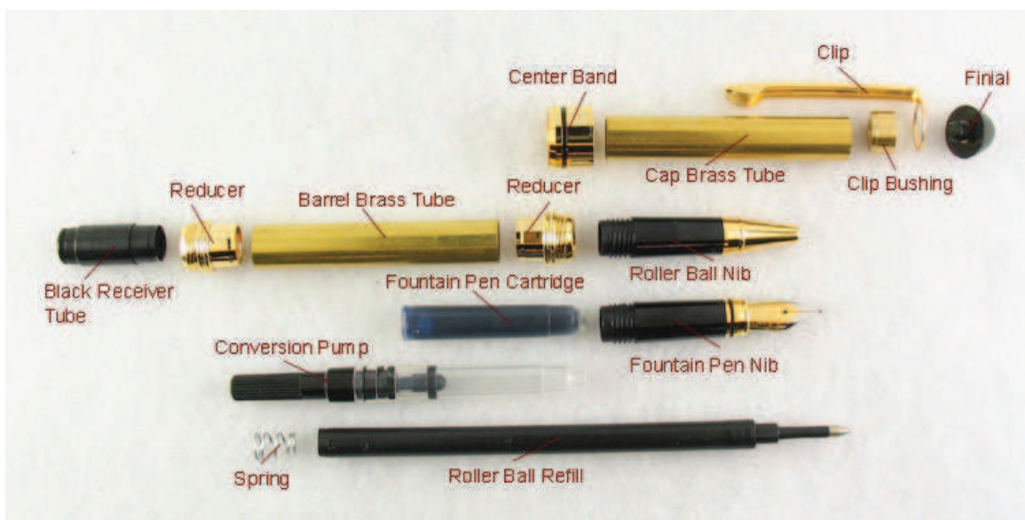
Parts Diagram
