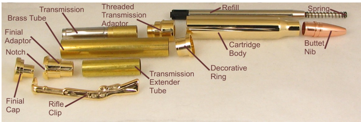
Parts Diagram
